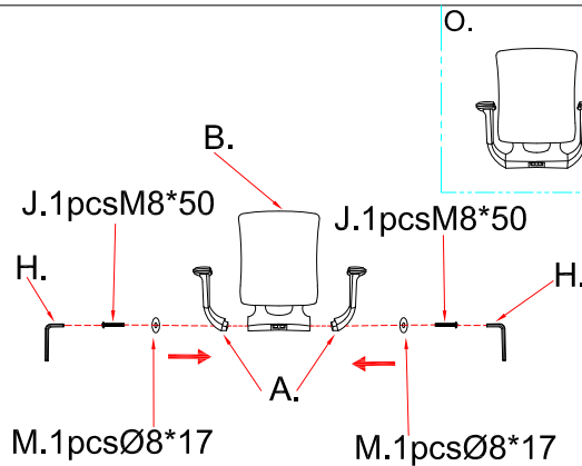
J.2pcsM8*50
